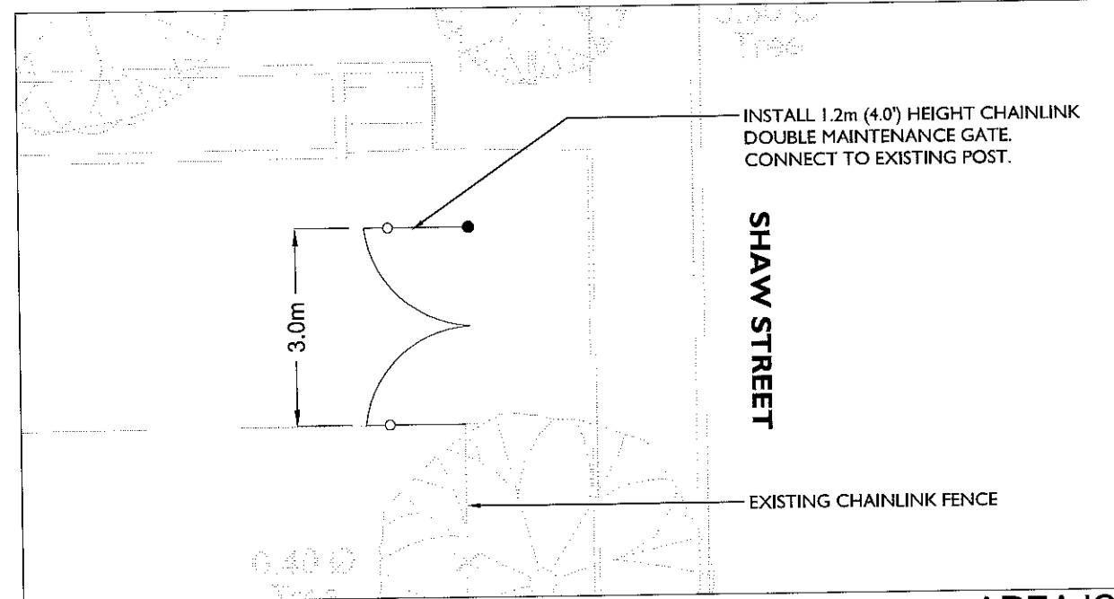
AREA 'C' 1:100
